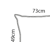
Cushion 1000043
